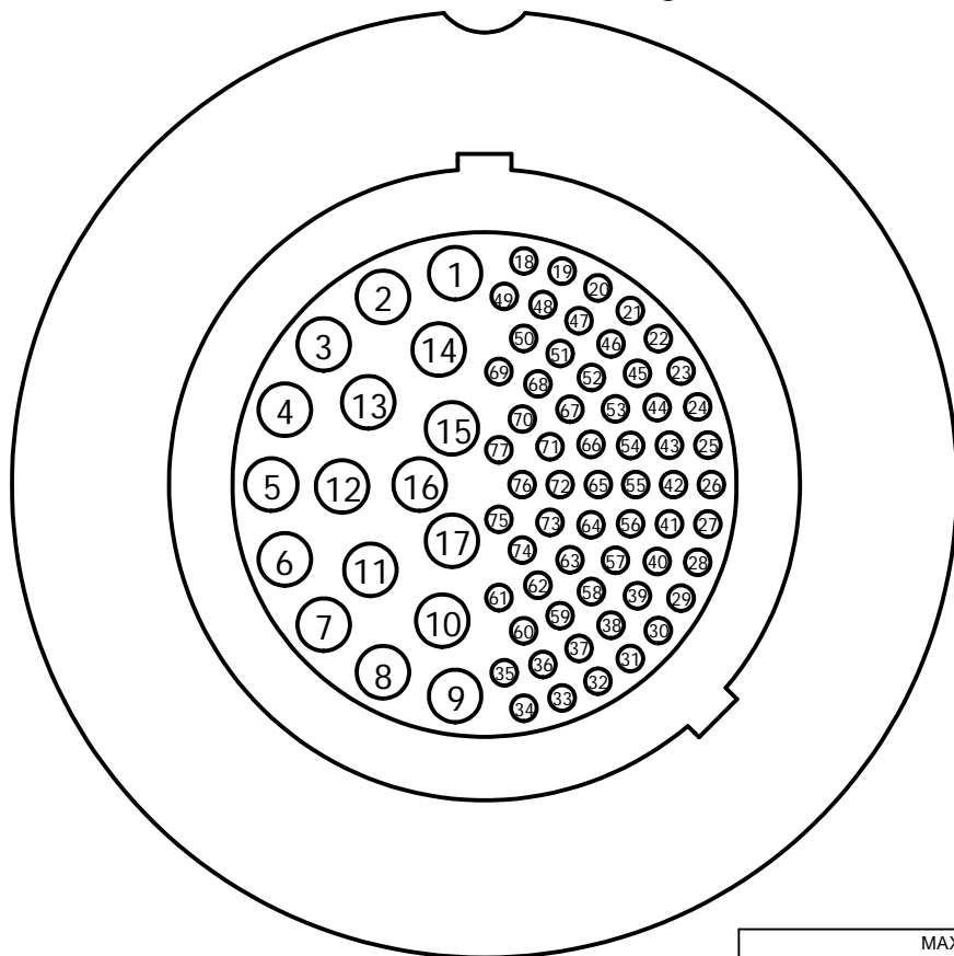
FACE VIEW
